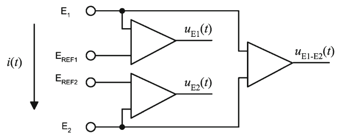
Fig. 1 Diagram of the measurement of the left electrode potential, the right electrode potential, difference of potentials between the left and the right electrodes, and the current flowing between the two electrodes
